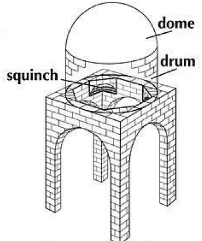
dome on squinches
