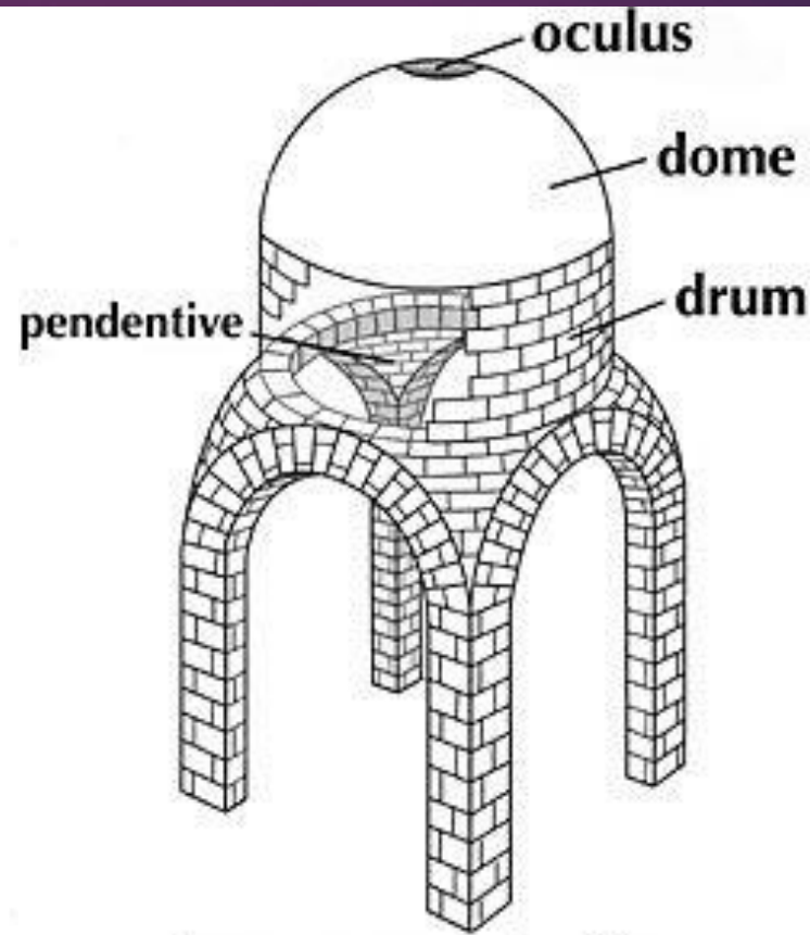
dome on pendentives
