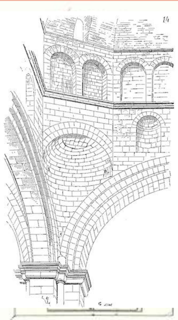
Corner SQUINCHES dome on squinches
